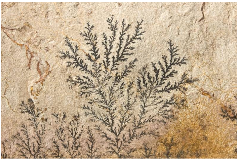
Dendritic manganese oxide minerals in Morocco. Width of view 7 cm.
